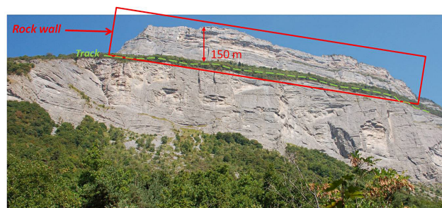
Fig. 5. Saint-Eynard calcareous cliff, near Grenoble.
